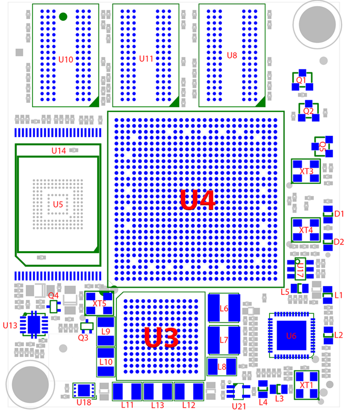
Figure 2. phyCORE-AM57x Component Placement (top view)
