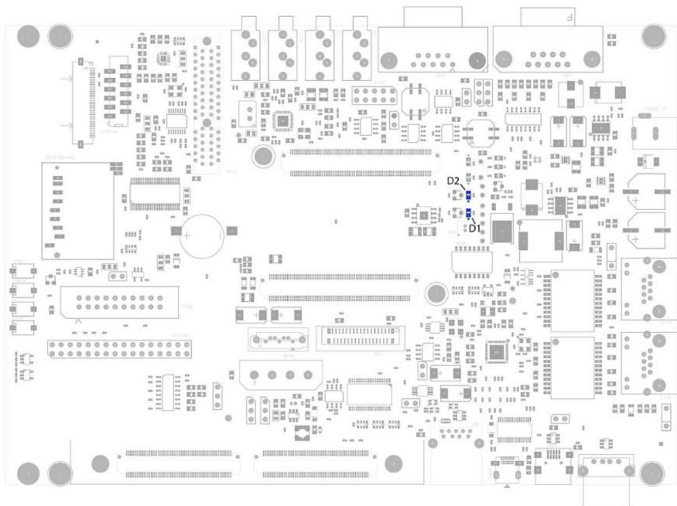
Figure 28. User LEDs
